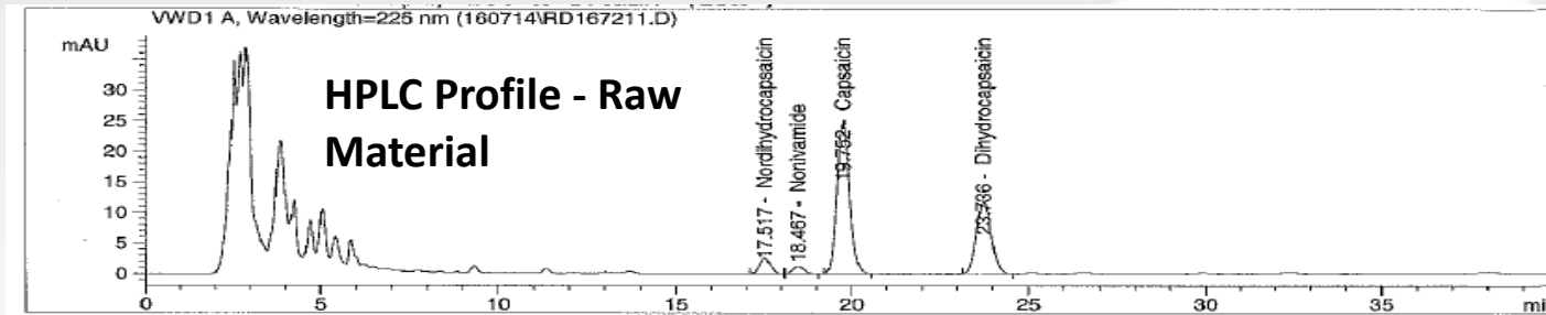
Capsaicin
