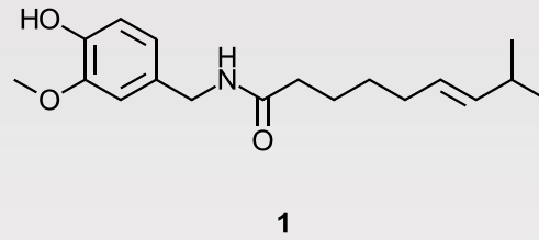
Capsaicin
